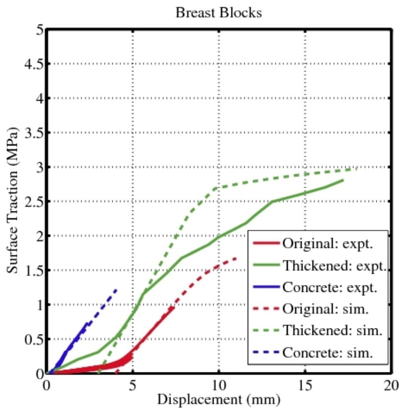
Figure 4. Surface traction versus displacement of breast blocks
