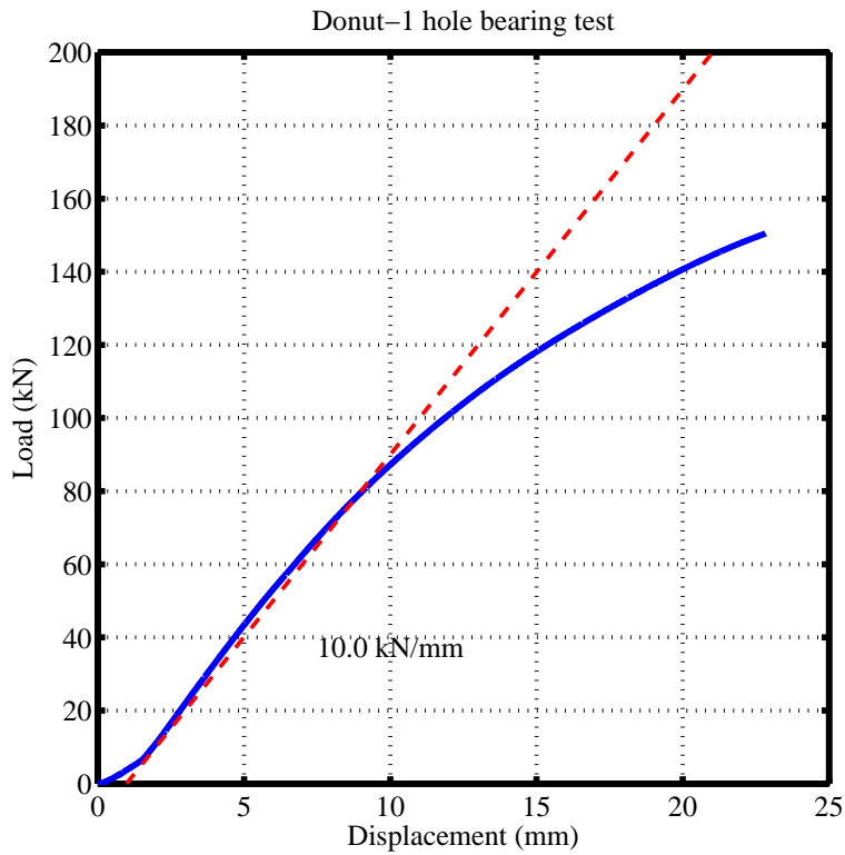
(a) Load vs. displacement.
